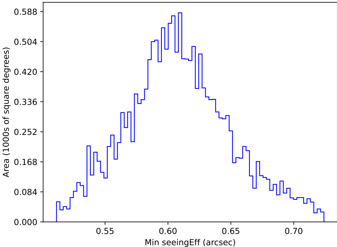
too_elab_2yr_r64_d3_ugrizy_v3.4_10yrs WFD z band: Min seeingEff
