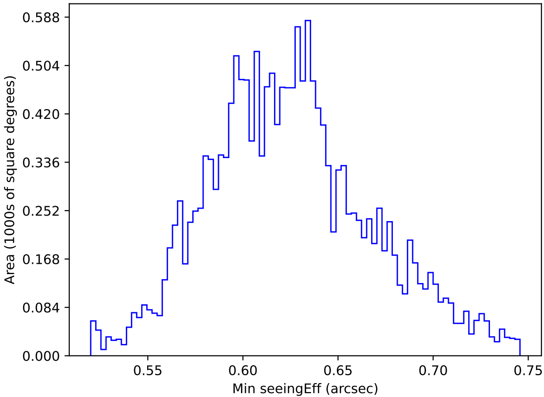
too_elab_2yr_r64_d3_ugrizy_v3.4_10yrs WFD y band: Min seeingEff
