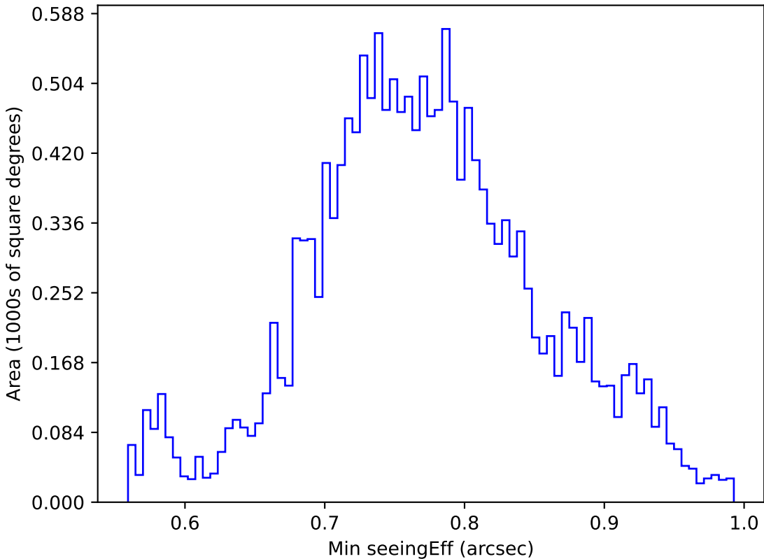
too_elab_2yr_r64_d3_ugrizy_v3.4_10yrs WFD u band: Min seeingEff
