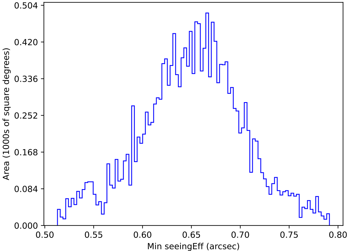
too_elab_2yr_r64_d3_ugrizy_v3.4_10yrs WFD g band: Min seeingEff
