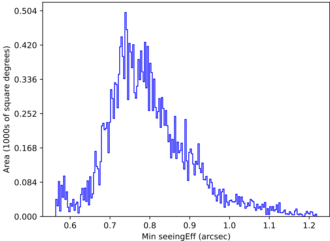
too_elab_2yr_r64_d3_ugrizy_v3.4_10yrs All sky u band: Min seeingEff
