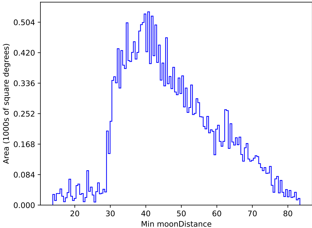
too_elab_2yr_r64_d3_ugrizy_v3.4_10yrs All sky g band: Min moonDistance
