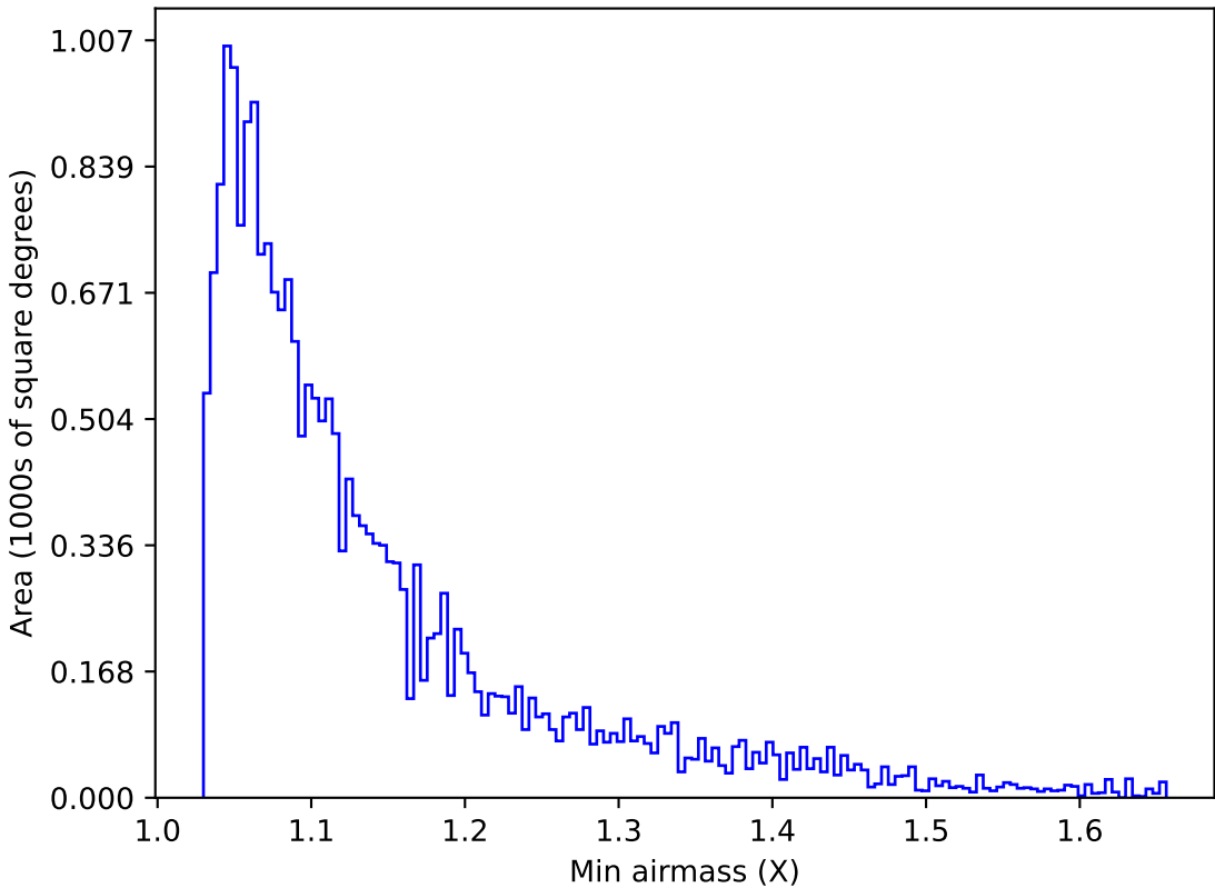
too_elab_2yr_r64_d3_ugrizy_v3.4_10yrs Yr 1 u band: Min airmass
