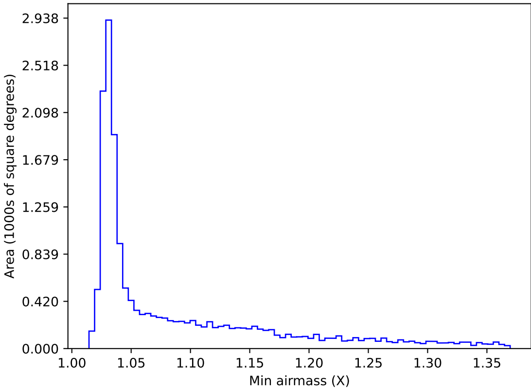
too_elab_2yr_r64_d3_ugrizy_v3.4_10yrs WFD y band: Min airmass
