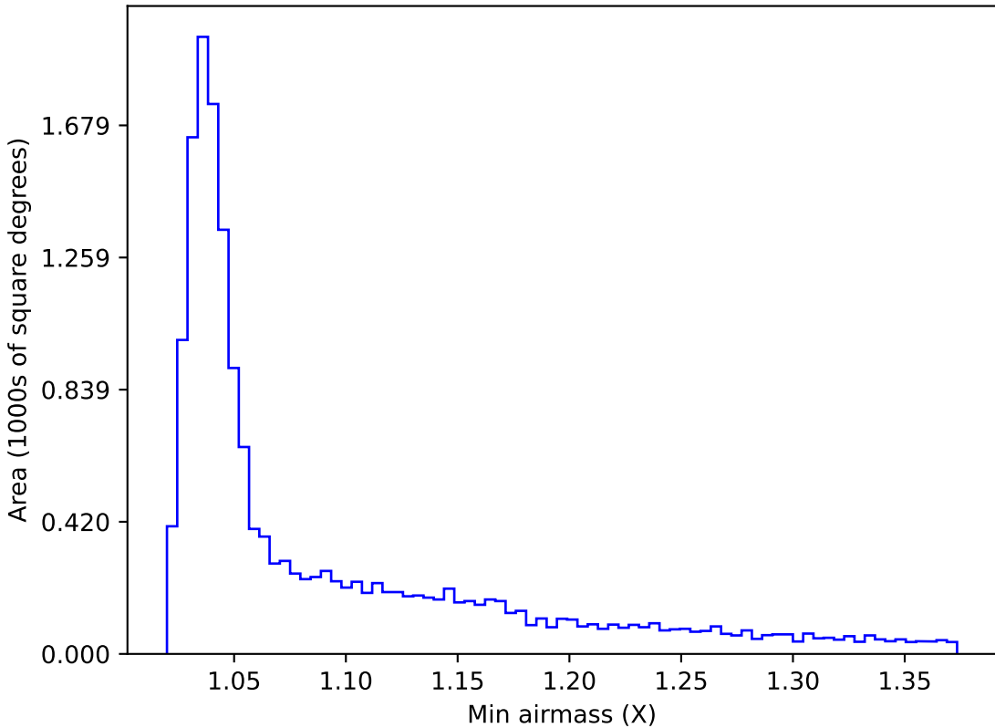
too_elab_2yr_r64_d3_ugrizy_v3.4_10yrs WFD u band: Min airmass
