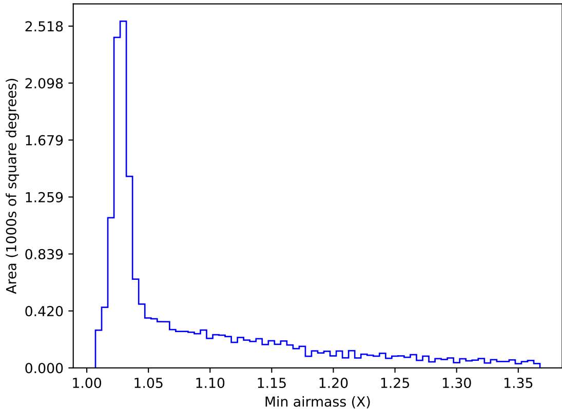
too_elab_2yr_r64_d3_ugrizy_v3.4_10yrs WFD r band: Min airmass
