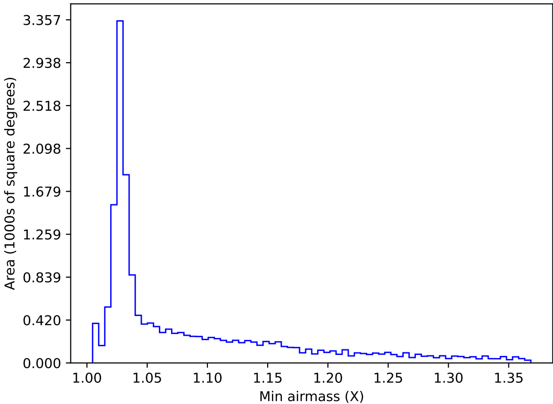
too_elab_2yr_r64_d3_ugrizy_v3.4_10yrs WFD i band: Min airmass
