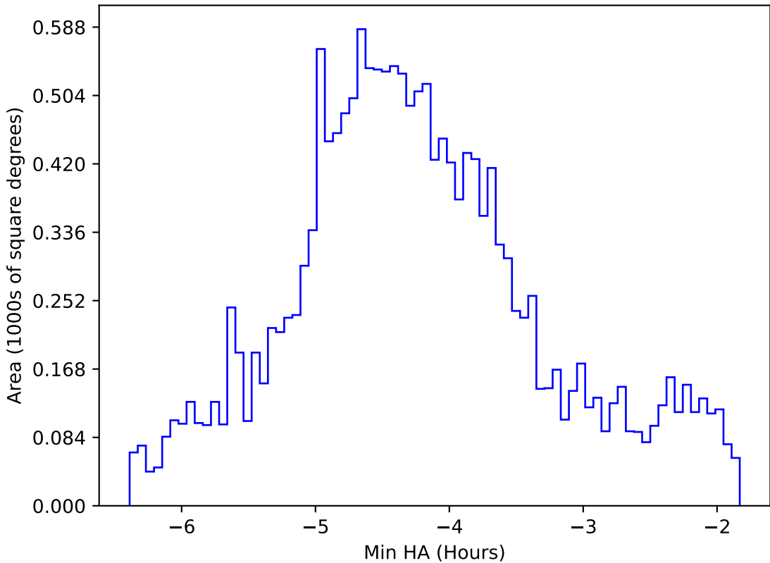
too_elab_2yr_r64_d3_ugrizy_v3.4_10yrs WFD g band: Min HA
