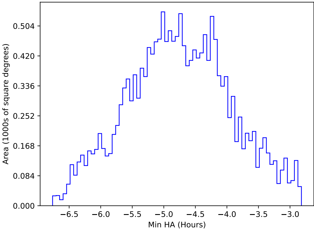
too_elab_2yr_r64_d3_ugrizy_v3.4_10yrs WFD all bands: Min HA
