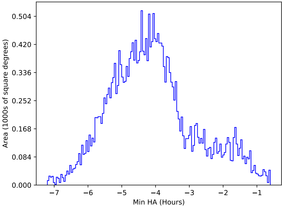
too_elab_2yr_r64_d3_ugrizy_v3.4_10yrs All sky z band: Min HA
