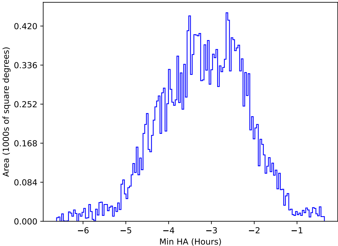
too_elab_2yr_r64_d3_ugrizy_v3.4_10yrs All sky u band: Min HA
