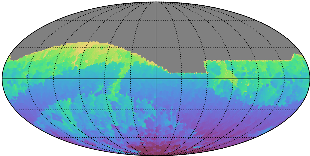
too_elab_2yr_r64_d3_ugrizy_v3.4_10yrs All sky r band: Min HA
