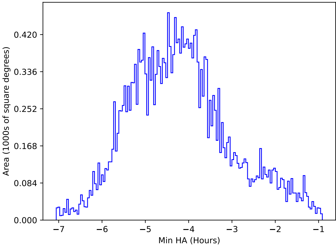
too_elab_2yr_r64_d3_ugrizy_v3.4_10yrs All sky r band: Min HA
