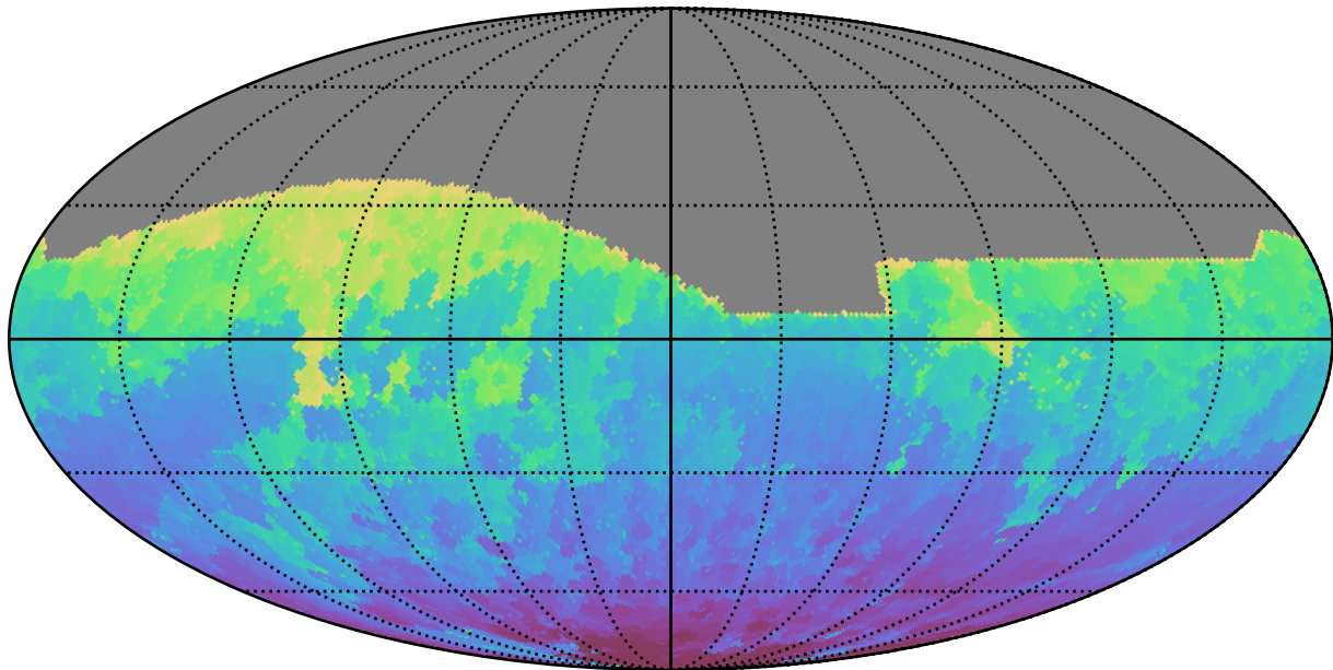
too_elab_2yr_r64_d3_ugrizy_v3.4_10yrs All sky i band: Min HA
