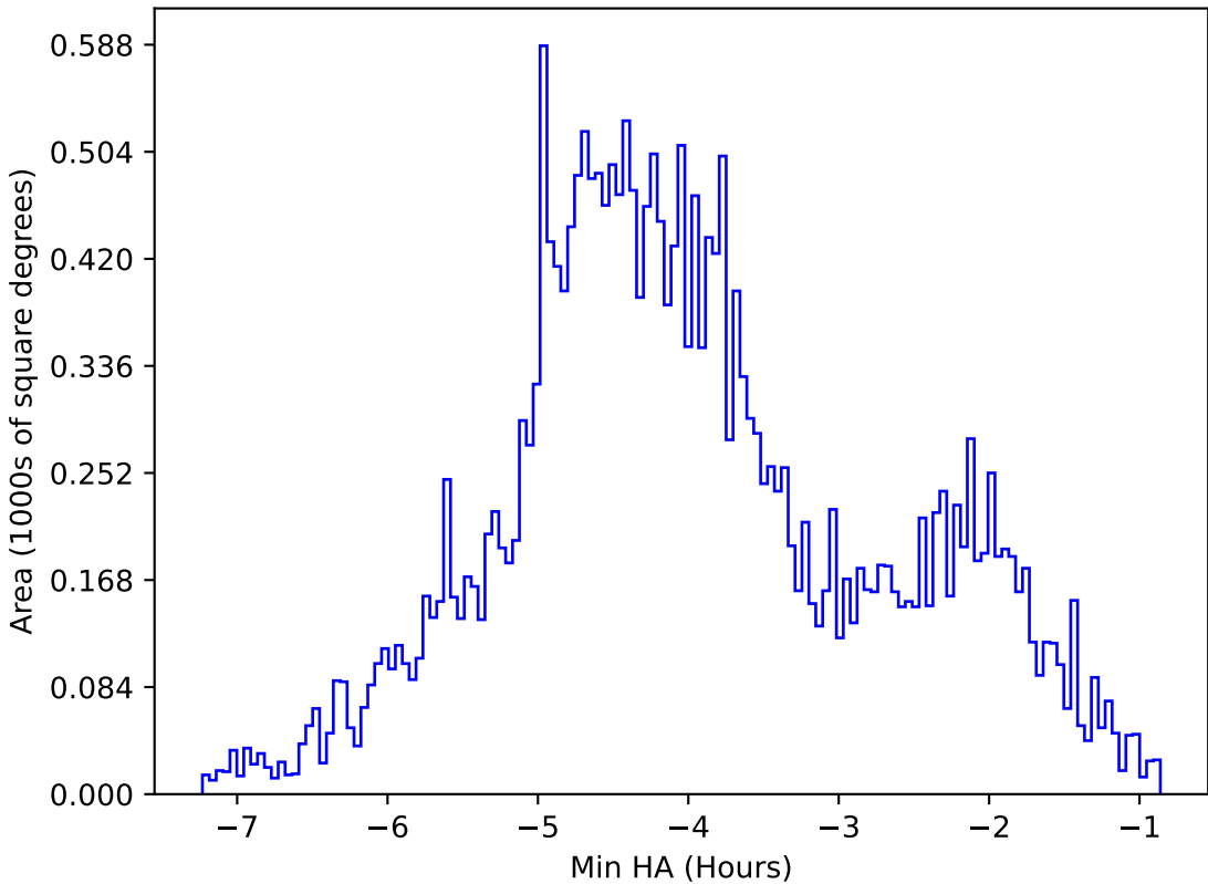
too_elab_2yr_r64_d3_ugrizy_v3.4_10yrs All sky g band: Min HA
