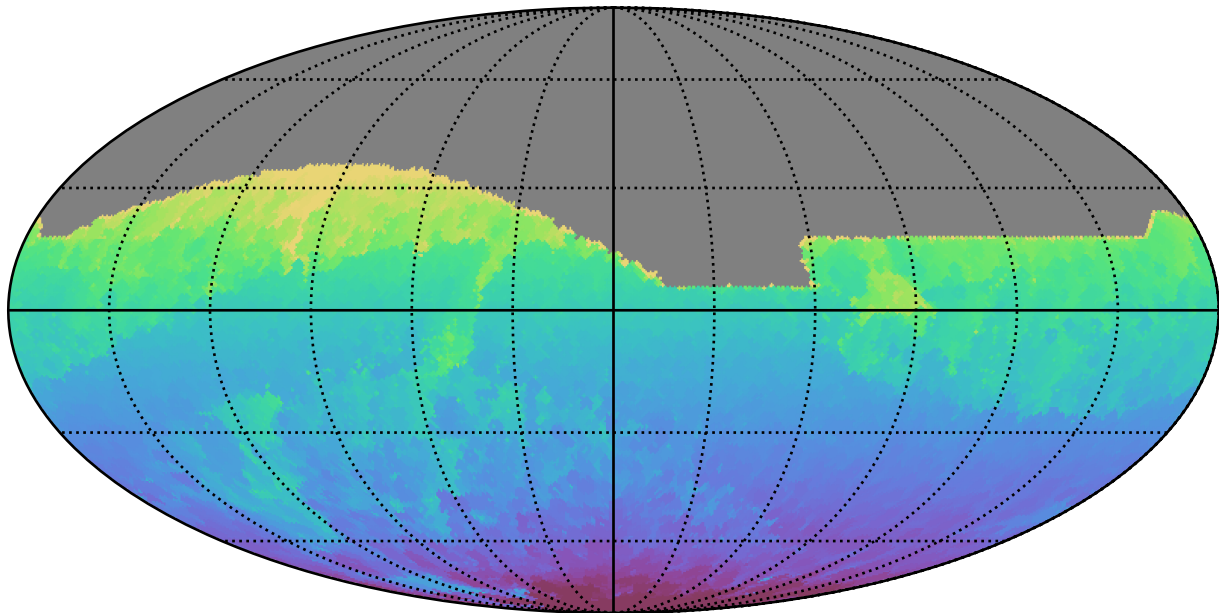
too_elab_2yr_r64_d3_ugrizy_v3.4_10yrs All sky all bands: Min HA
