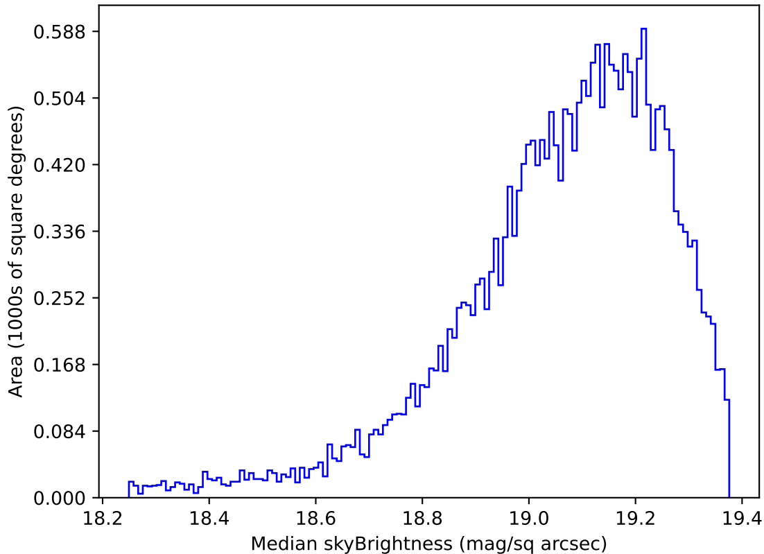
too_elab_2yr_r64_d3_ugrizy_v3.4_10yrs Yr 1 z band: Median skyBrightness
