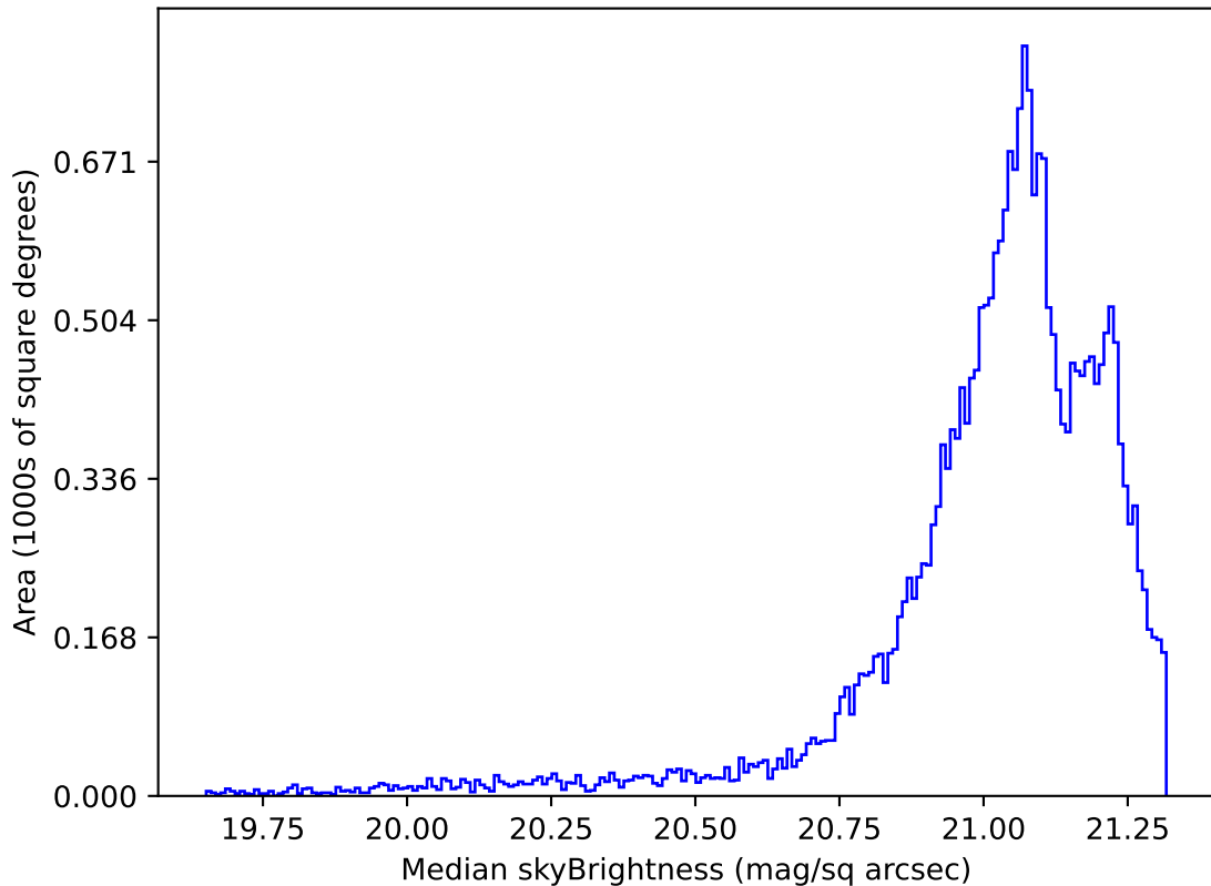
too_elab_2yr_r64_d3_ugrizy_v3.4_10yrs Yr 1 r band: Median skyBrightness
