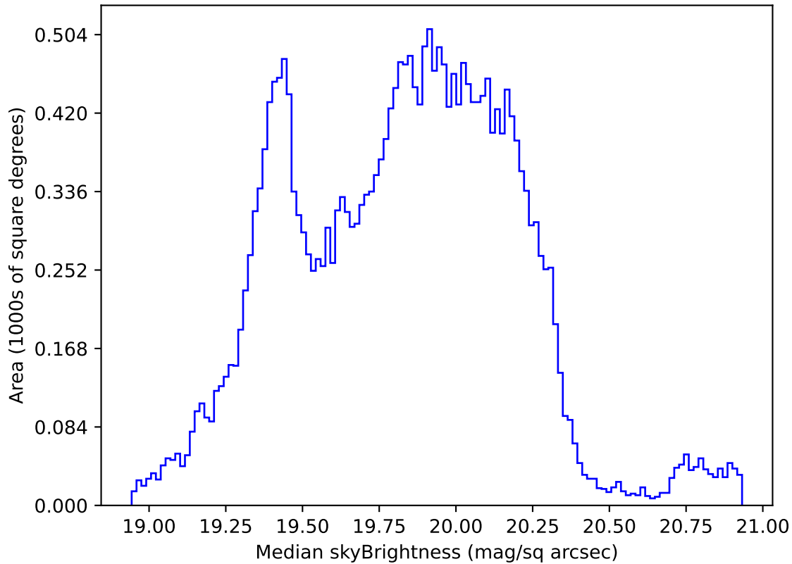
too_elab_2yr_r64_d3_ugrizy_v3.4_10yrs Yr 1 all bands: Median skyBrightness
