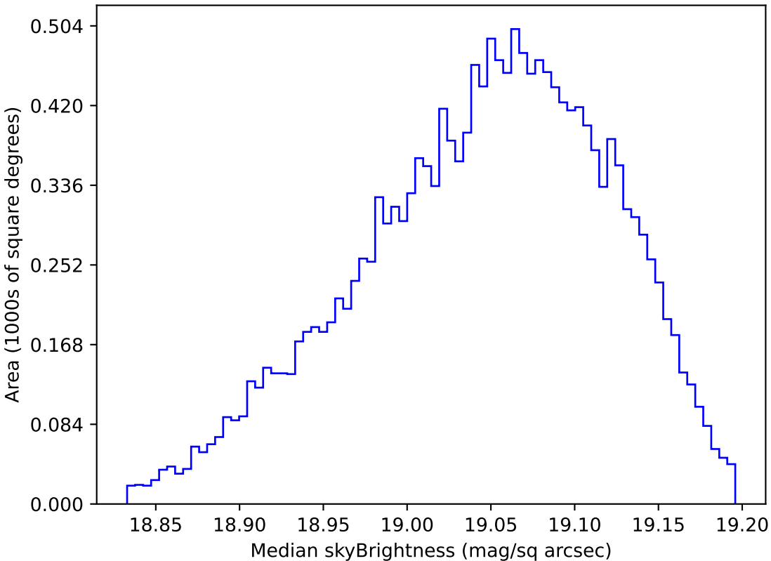
too_elab_2yr_r64_d3_ugrizy_v3.4_10yrs WFD z band: Median skyBrightness
