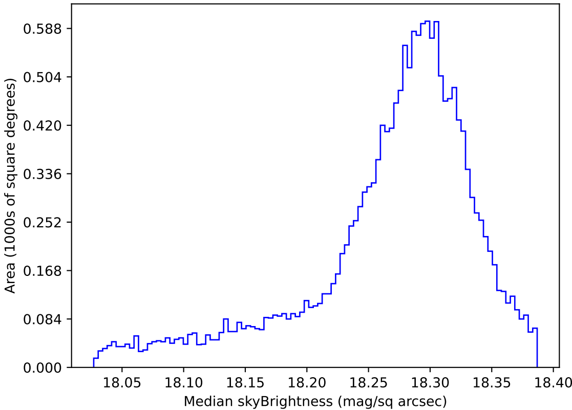
too_elab_2yr_r64_d3_ugrizy_v3.4_10yrs WFD y band: Median skyBrightness
