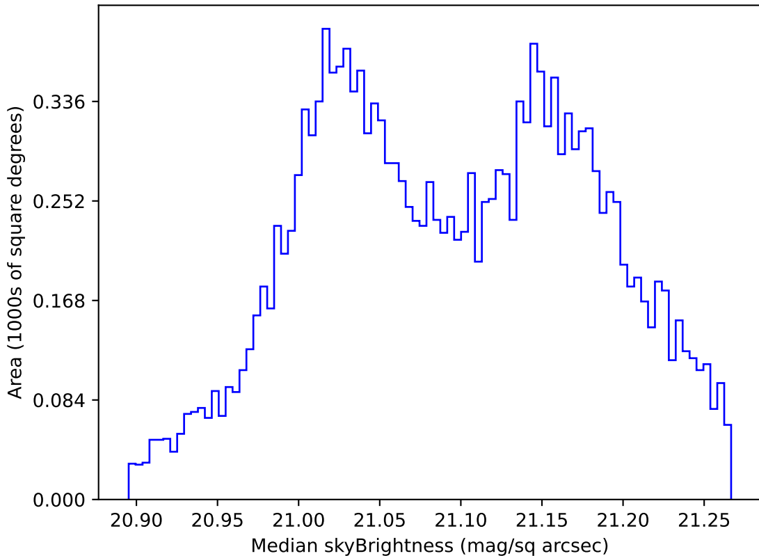
too_elab_2yr_r64_d3_ugrizy_v3.4_10yrs WFD r band: Median skyBrightness
