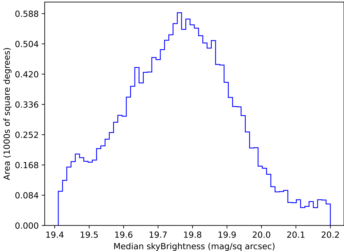
too_elab_2yr_r64_d3_ugrizy_v3.4_10yrs WFD all bands: Median skyBrightness
