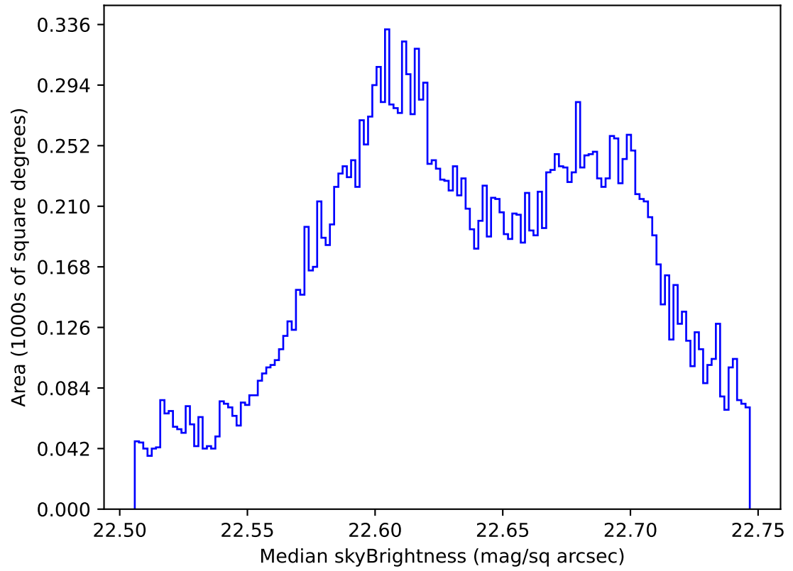
too_elab_2yr_r64_d3_ugrizy_v3.4_10yrs All sky u band: Median skyBrightness
