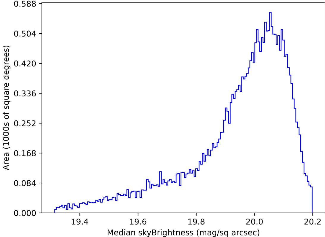
too_elab_2yr_r64_d3_ugrizy_v3.4_10yrs All sky i band: Median skyBrightness
