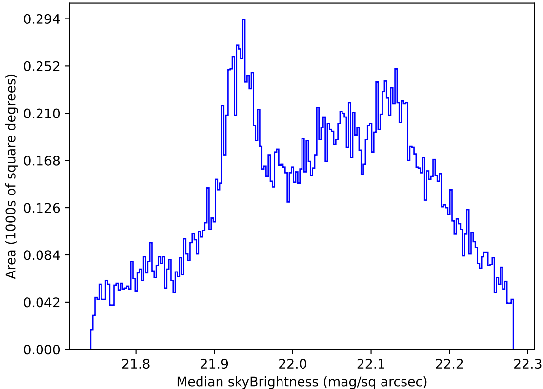
too_elab_2yr_r64_d3_ugrizy_v3.4_10yrs All sky g band: Median skyBrightness
