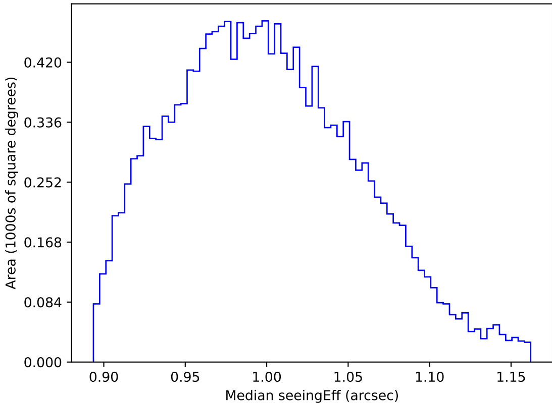
too_elab_2yr_r64_d3_ugrizy_v3.4_10yrs WFD y band: Median seeingEff
