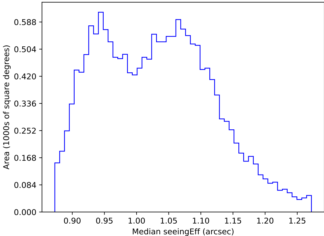
too_elab_2yr_r64_d3_ugrizy_v3.4_10yrs WFD r band: Median seeingEff
