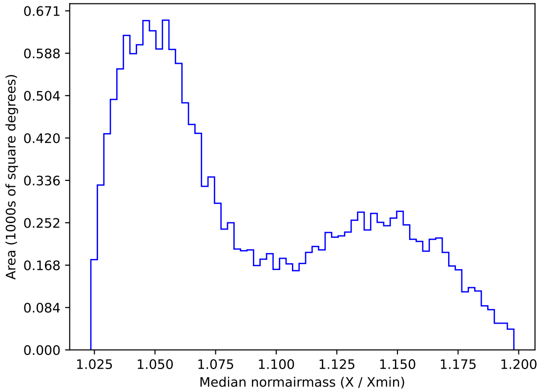
too_elab_2yr_r64_d3_ugrizy_v3.4_10yrs WFD z band: Median normairmass
