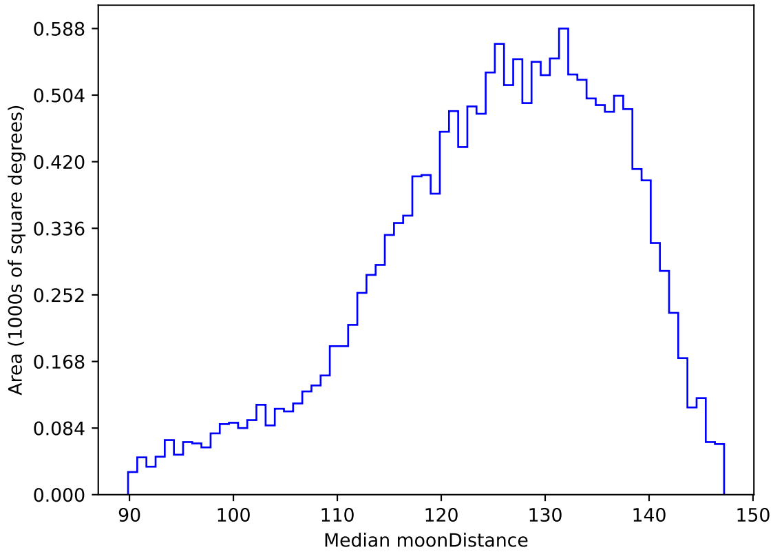
too_elab_2yr_r64_d3_ugrizy_v3.4_10yrs WFD u band: Median moonDistance
