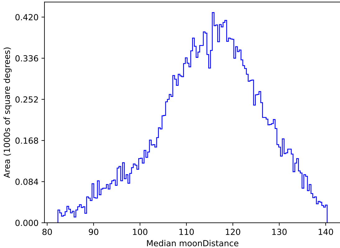
too_elab_2yr_r64_d3_ugrizy_v3.4_10yrs All sky g band: Median moonDistance
