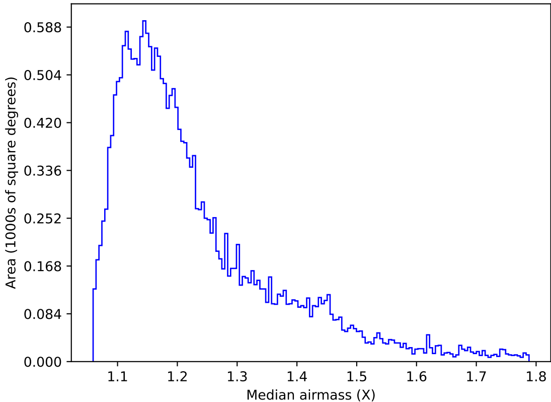
too_elab_2yr_r64_d3_ugrizy_v3.4_10yrs Yr 1 u band: Median airmass
