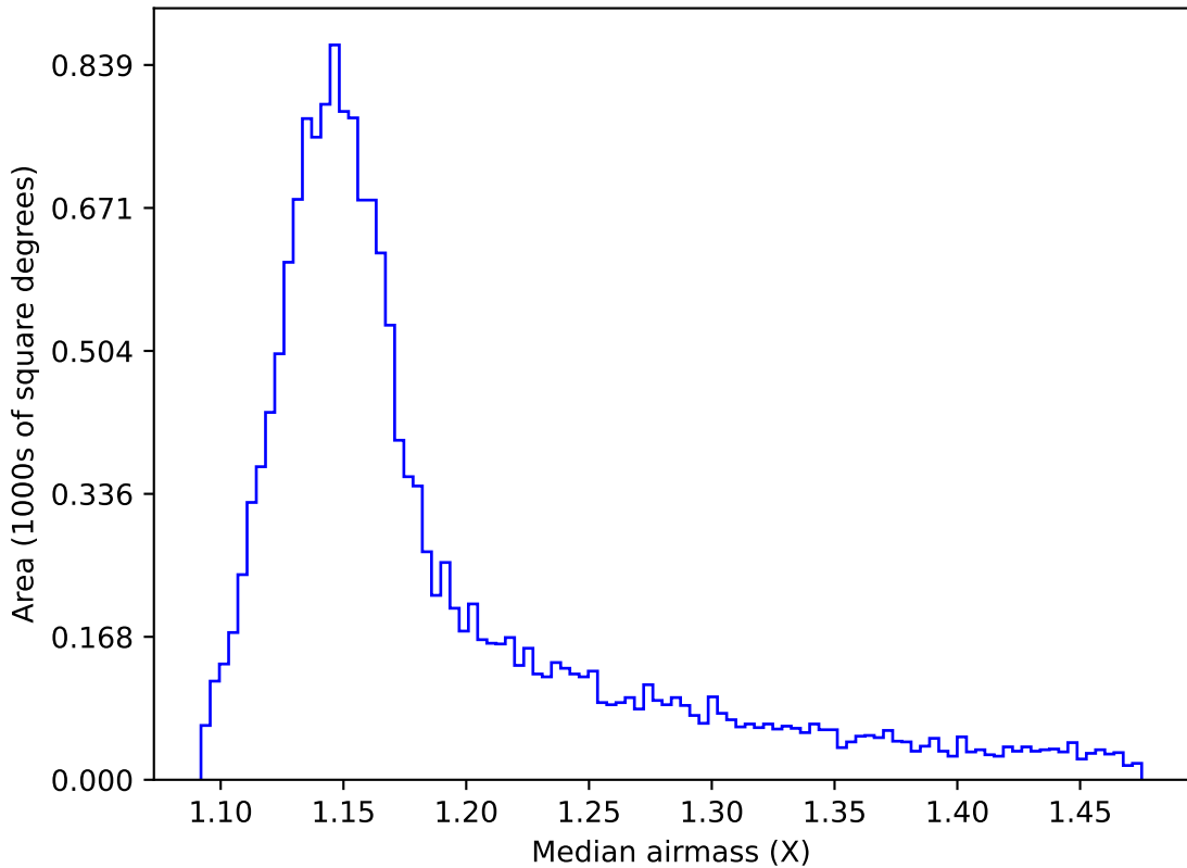
too_elab_2yr_r64_d3_ugrizy_v3.4_10yrs WFD y band: Median airmass
