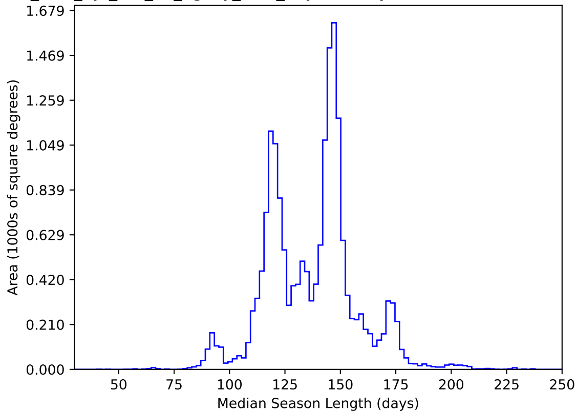
too_elab_2yr_r64_d3_ugrizy_v3.4_10yrs WFD y band: Median Season Length
