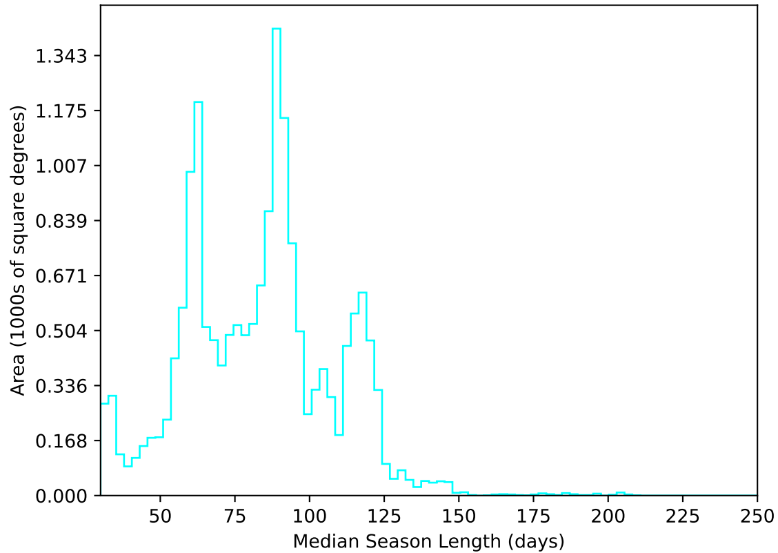
too_elab_2yr_r64_d3_ugrizy_v3.4_10yrs WFD u band: Median Season Length
