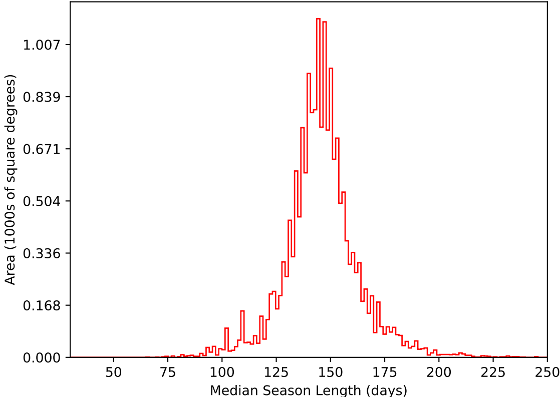
too_elab_2yr_r64_d3_ugrizy_v3.4_10yrs WFD i band: Median Season Length
