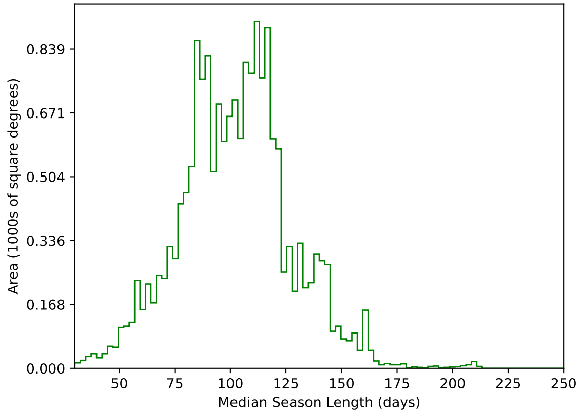
too_elab_2yr_r64_d3_ugrizy_v3.4_10yrs WFD g band: Median Season Length
