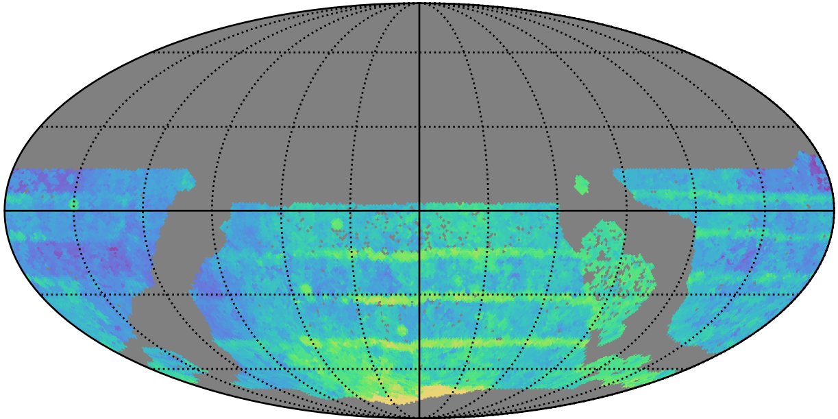
too_elab_2yr_r64_d3_ugrizy_v3.4_10yrs WFD all bands: Median Season Length
