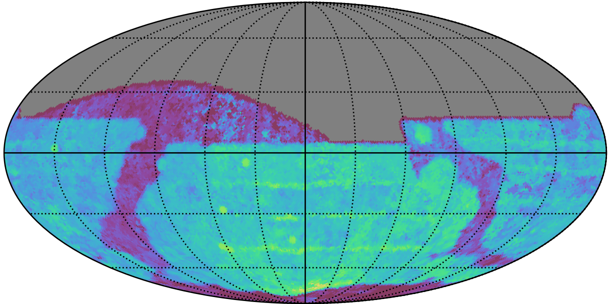
too_elab_2yr_r64_d3_ugrizy_v3.4_10yrs All sky z band: Median Season Length
