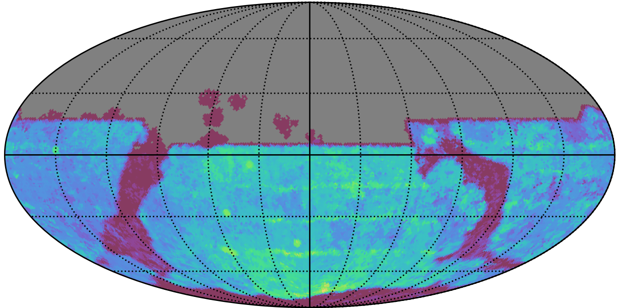
too_elab_2yr_r64_d3_ugrizy_v3.4_10yrs All sky y band: Median Season Length
