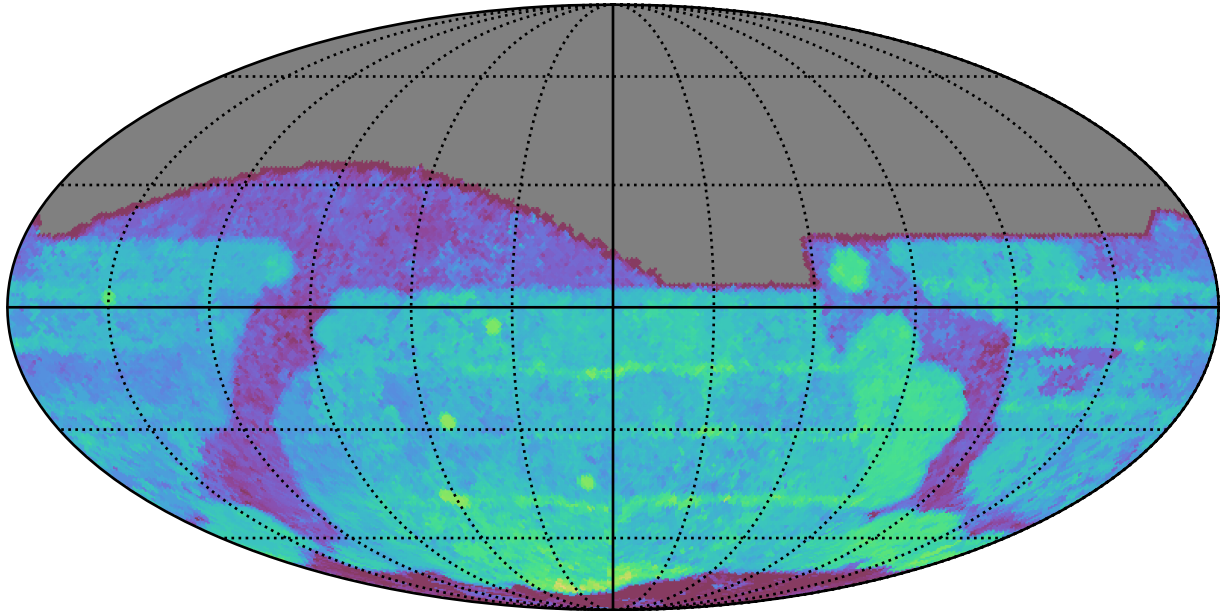
too_elab_2yr_r64_d3_ugrizy_v3.4_10yrs All sky r band: Median Season Length
