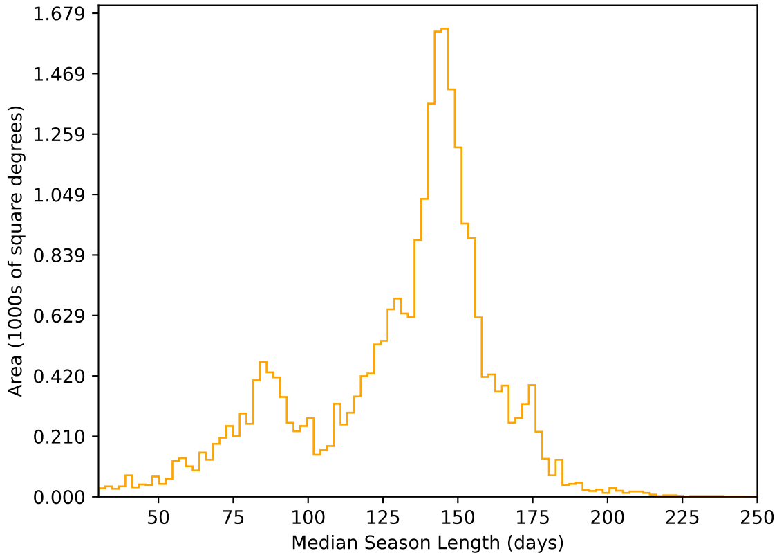
too_elab_2yr_r64_d3_ugrizy_v3.4_10yrs All sky r band: Median Season Length
