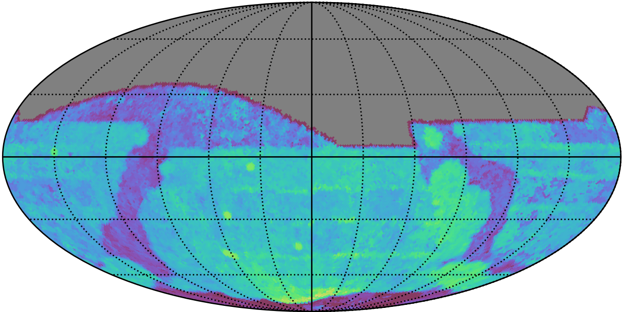
too_elab_2yr_r64_d3_ugrizy_v3.4_10yrs All sky i band: Median Season Length
