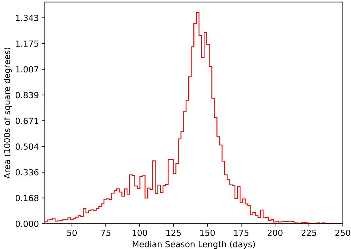
too_elab_2yr_r64_d3_ugrizy_v3.4_10yrs All sky i band: Median Season Length
