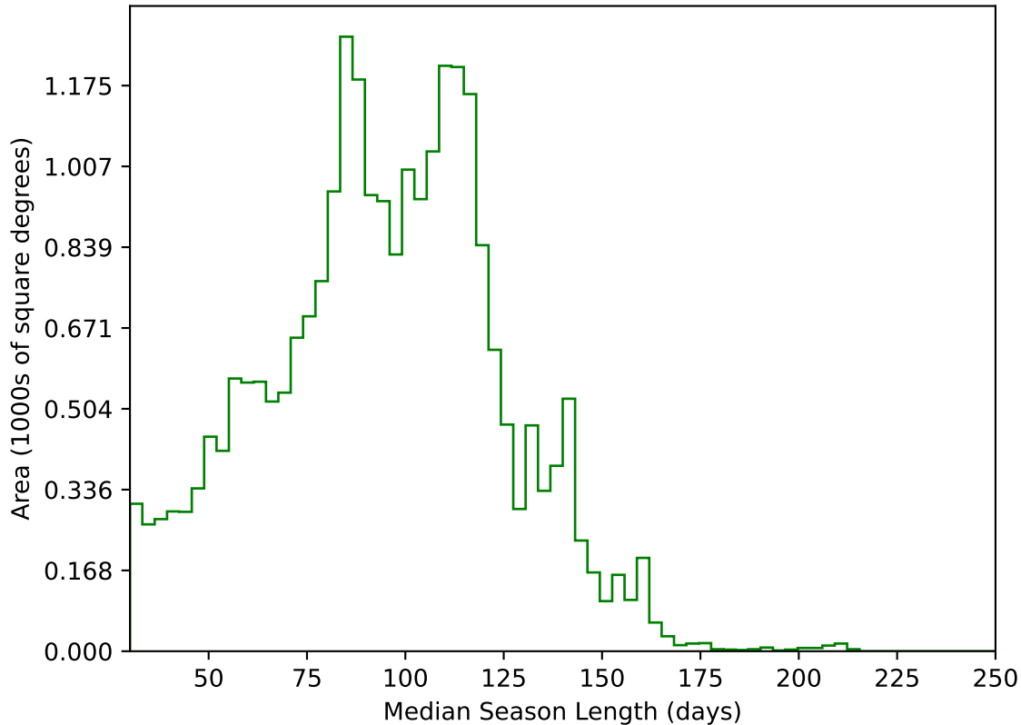
too_elab_2yr_r64_d3_ugrizy_v3.4_10yrs All sky g band: Median Season Length
