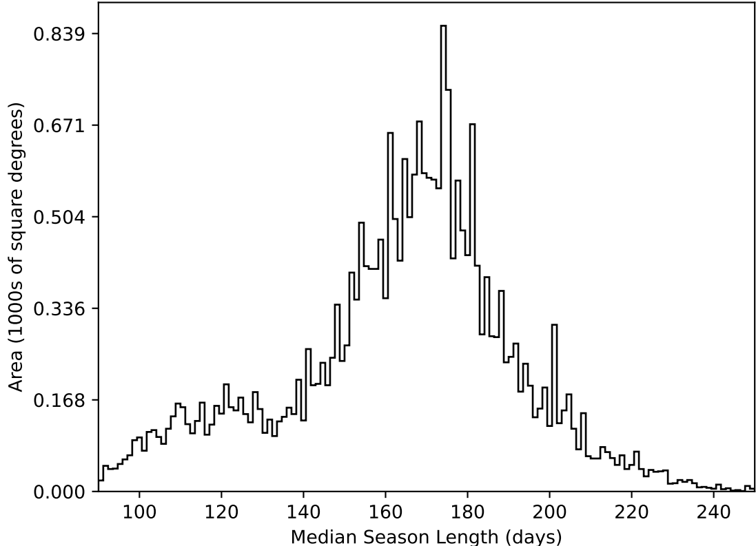
too_elab_2yr_r64_d3_ugrizy_v3.4_10yrs All sky all bands: Median Season Length
